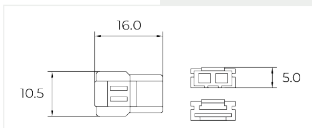
SELF CONNECT ADAPTER - FOR 8MM STRIP LIGHT
