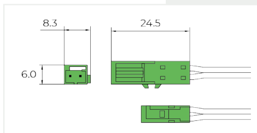
EXTENSION CABLE - WITH TINNED ENDS
