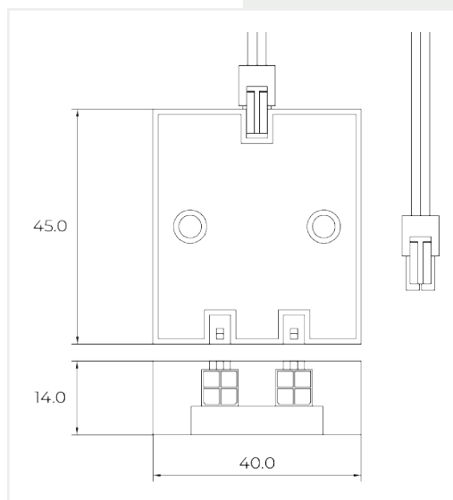
2 PORT SENSOR SPLITTER - WITH ACCESSORY PORT CONNECTION
