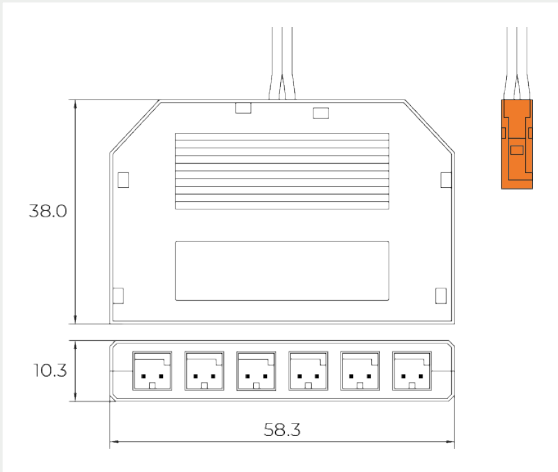
6 WAY SPLITTER SOCKET - WITH SYNDEO CONNECTION
