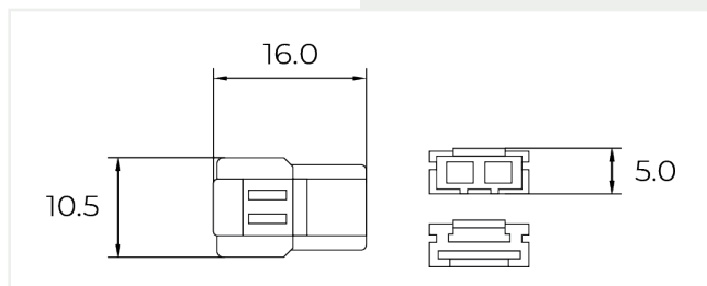
SELF CONNECT ADAPTER - FOR 8MM STRIP LIGHT
